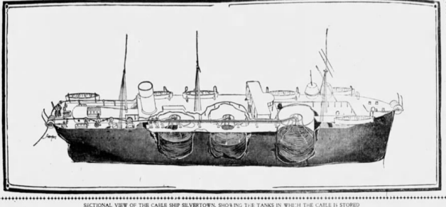
SECTIONAL VIEW OF THE CABLE SHIP SILVERTON, SHOWING THE TANKS IN WHICH THE CABLE IS STORED
